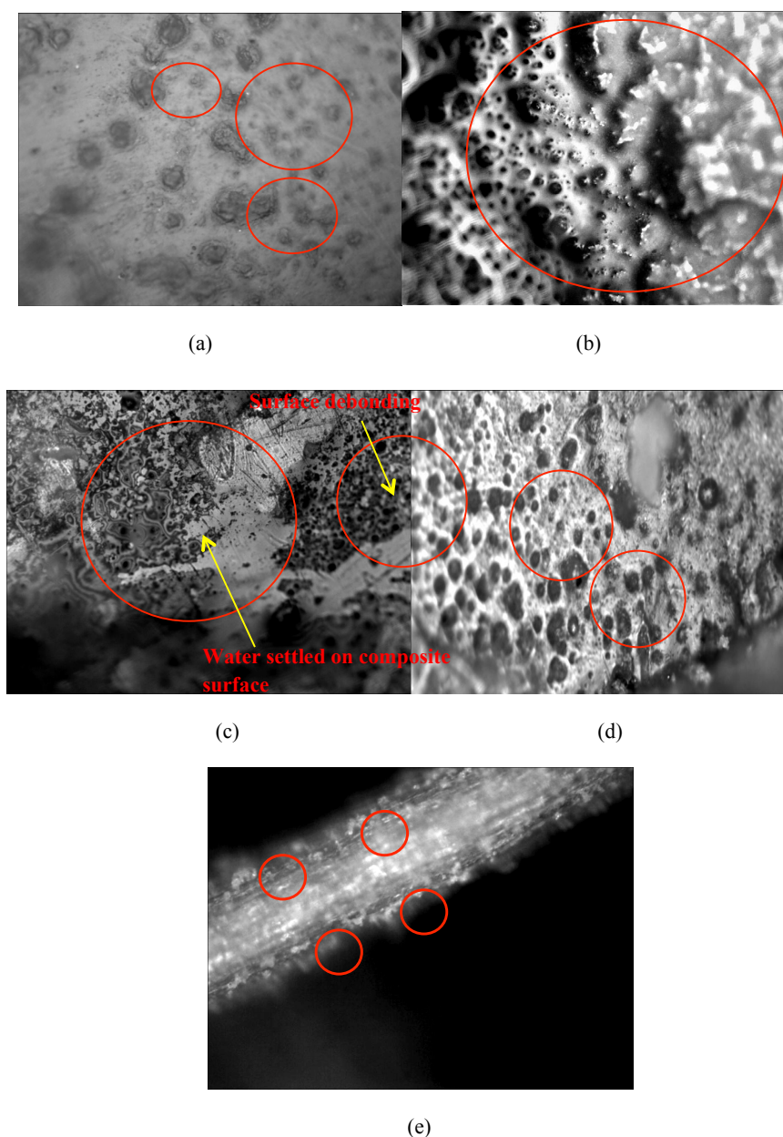
Figure 9. Microstructure analysis of composite samples (a) Sawdust agglomeration at higher filler percentage, (b) Non-uniform wetting at lower matrix percentage, (c) Water settled on uneven composite surface after ageing, resulting in surface debonding, (d) Pores formed on composite surfaces (e) Salt settled on fibre surface
